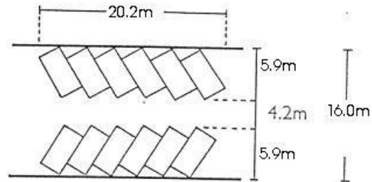
60° PARKING
