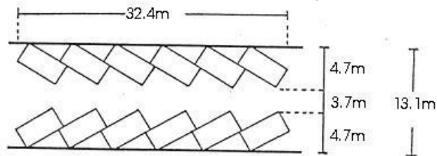
30° PARKING
