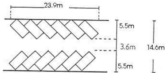
45° PARKING
