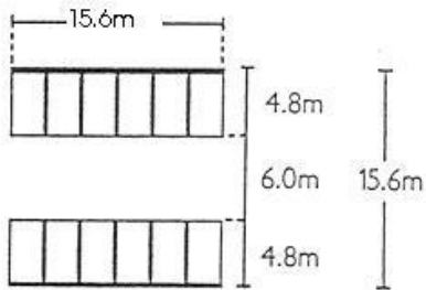
90° PARKING
