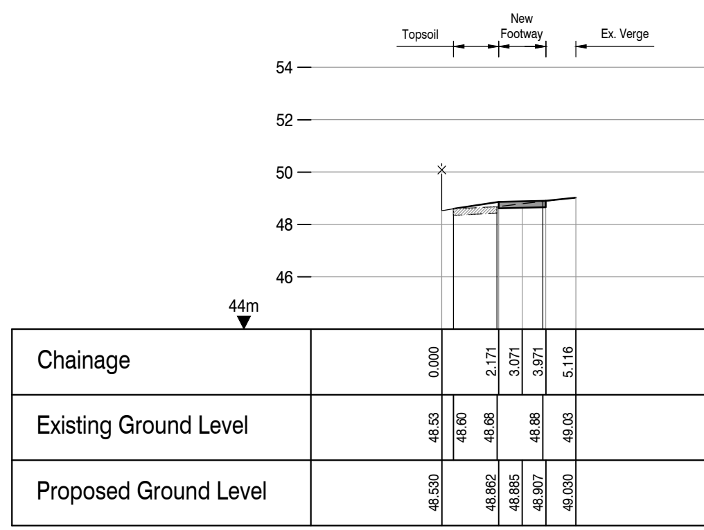
CROSS SECTION - CHAINAGE 30m
