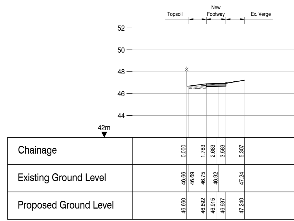
CROSS SECTION - CHAINAGE 75m
