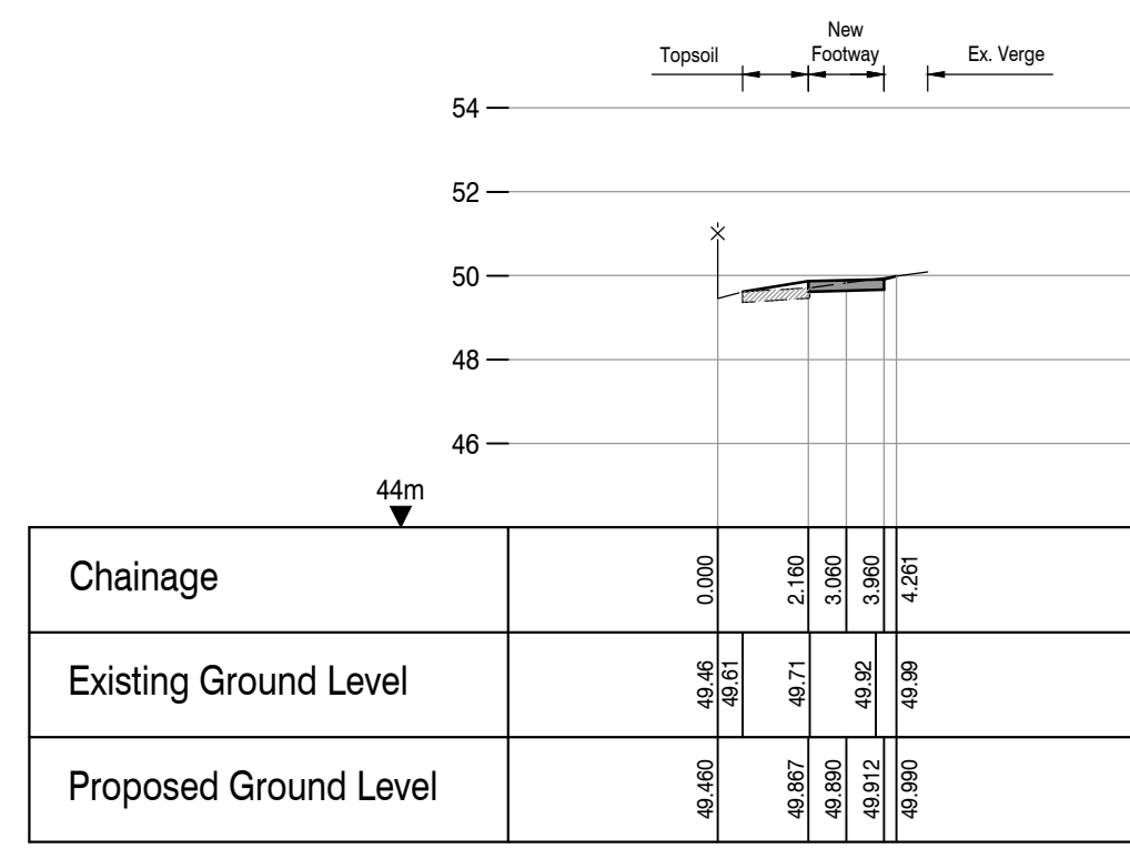
CROSS SECTION - CHAINAGE 15m
