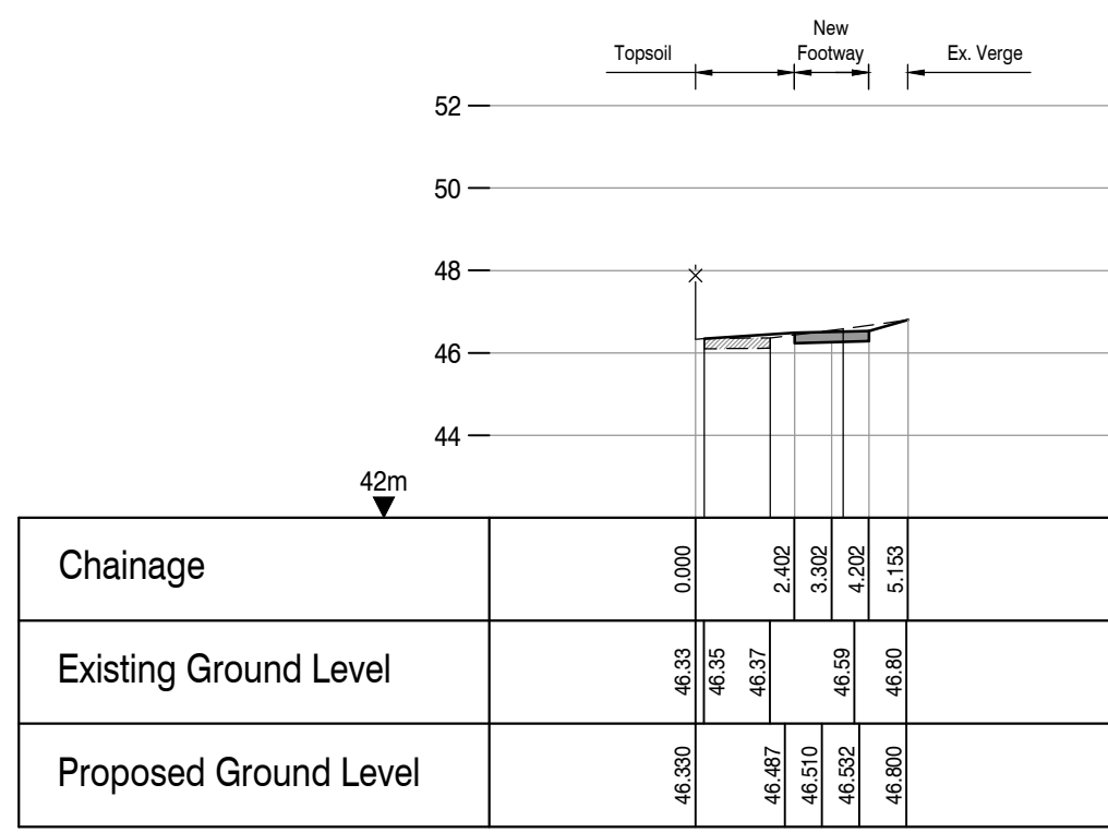
CROSS SECTION - CHAINAGE 90m
