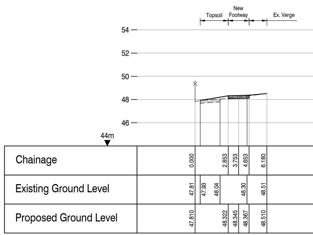
CROSS SECTION - CHAINAGE 45m
