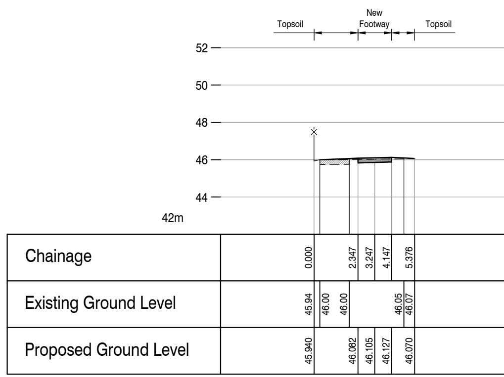
CROSS SECTION - CHAINAGE 105m
