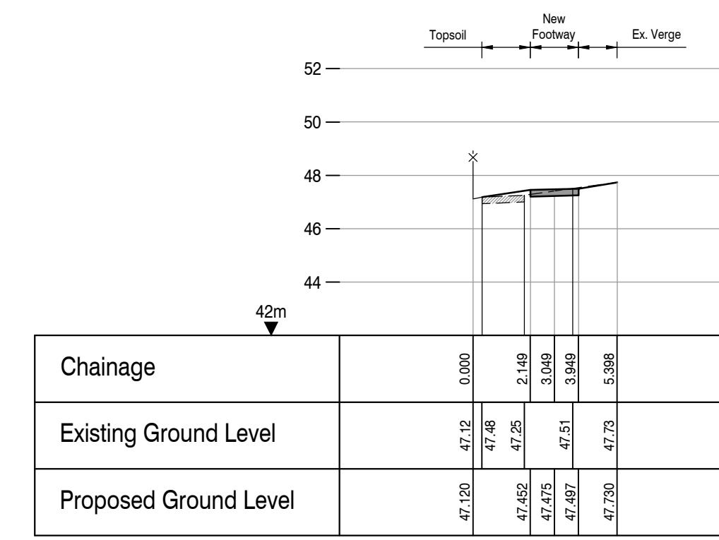
CROSS SECTION - CHAINAGE 60m
