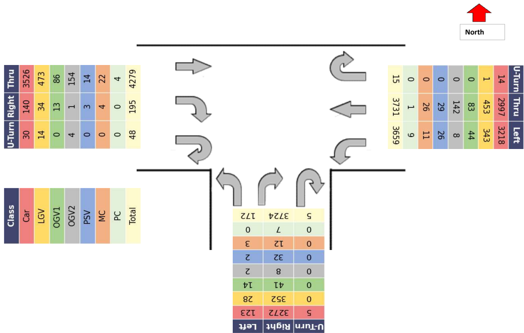
Turning Movement Data Plot
