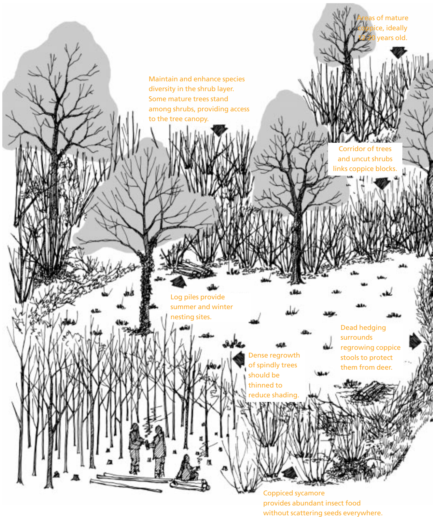
Figure 2 Features of good dormouse habitat management. The best habitat for dormice is in actively coppiced ancient woodland that maintains a rich herb and shrub layer below an open canopy.
