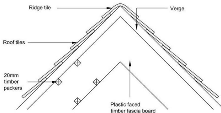
SECTION: ROOST OPPORTUNITY BEHIND FASCIA BOARD Not to scale
