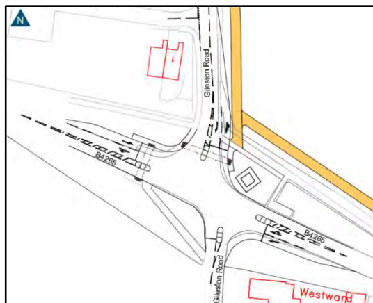
Figure 1: J18 Potential Signal Control Arrangement (source - Lime Transport TA 22087d1a)
